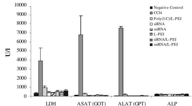
Fig. 7. Level of hepatic enzymes after siRNA/L-PEI and ssiRNA/L-PEI complex injection in mice serum. Forty micrograms of siRNAs or ssiRNAs complexed with L-PEI (N/P=8) were injected i.v. L-PEI alone (6.4 \mu l, corresponding to N/P=8), siRNAs alone (40 \mu g) and ssiRNAs alone (40 \mu g) were also injected. As a negative control, 5% Glucose solution was used. As positive controls 50 \mu g of E. coli LPS in PBS was injected i.p. and CCl 4 , (12.5 in 100 \mu l olive oil) was s.c. administrated. Twenty-four hours after injection, blood was collected. The level of hepatic enzyme (Alanine aminotransferase, SGPT or ALAT, Aspartate aminotransferase, SGOT or ASAT, Alkaline phosphatase, ALP, and Lactate dehydrogenase, LDH) was determined on serum. Each value represents the mean \pm SD ( n=4 for controls and n=8 for specific assays).
